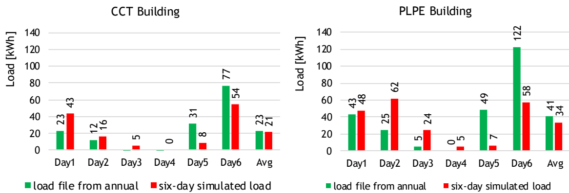
Fig. 4: Comparison of daily loads defined in the CCT and PLPE methods.
